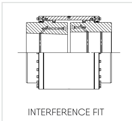
INTERFERENCE WITH INTERMEDIATE CONICAL BUSHING
