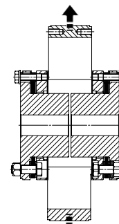
Split spacer
