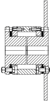
DMUCCBD WITH INTEGRATED BRAKE DISC
