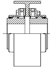
FBP/FSUBP BRAKE PULLEY C4266a Page 44
